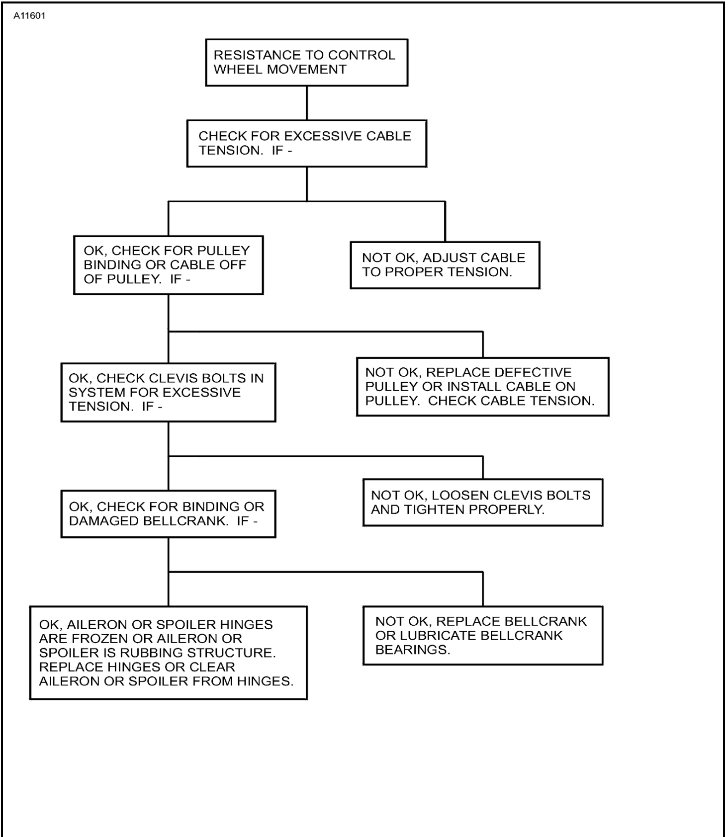
Figure 101 : Sheet 2 : Aileron and Control System Troubleshooting Chart
